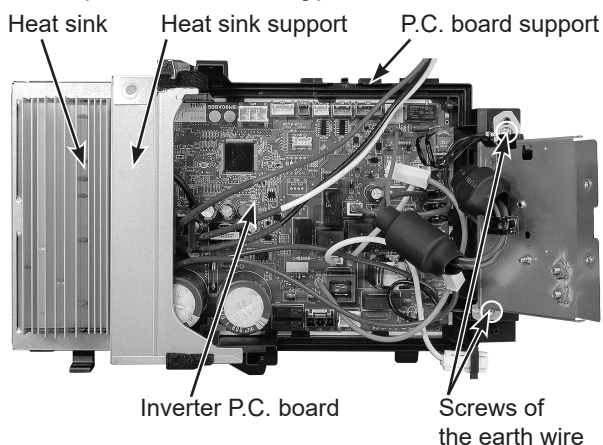
Photo 6 (Inverter assembly)
