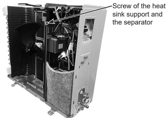
Photo 6 (Inverter assembly)
