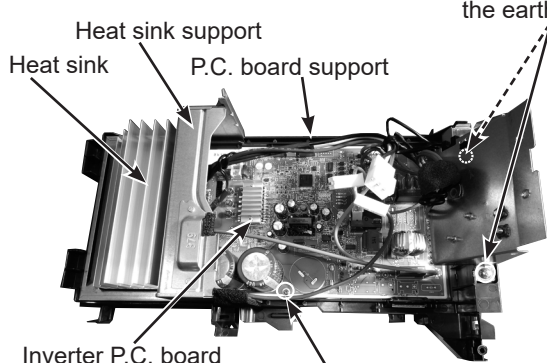
Photo 6 (Inverter assembly)
