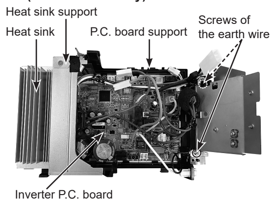
Photo 5 (Inverter assembly)
