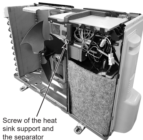
Photo 5 (Inverter assembly)
