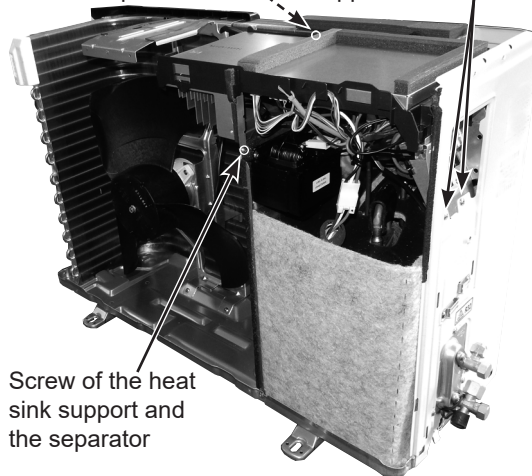
Photo 6 (Inverter assembly)
