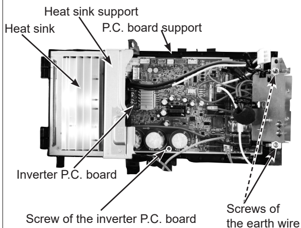
Photo 4 (Inverter assembly)
