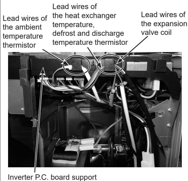
Photo 5 (Inverter assembly)
