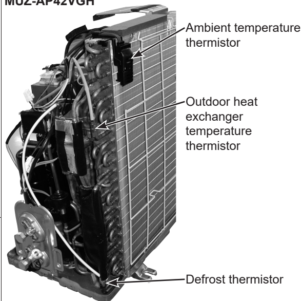
MUZ-AP42VGH
