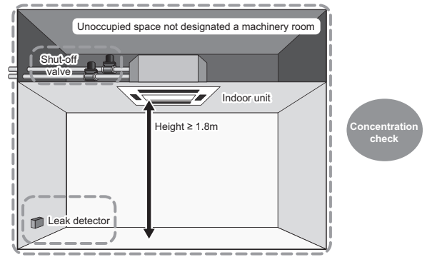
(2-6) Small room installation (Shut-off valves)
