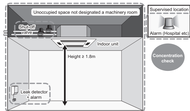
(2-3) Small room installation (Alarm + Shut-off valves)
