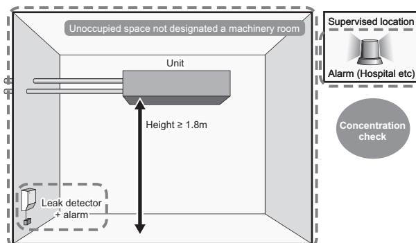
(1-3) Small room installation (Alarm)
