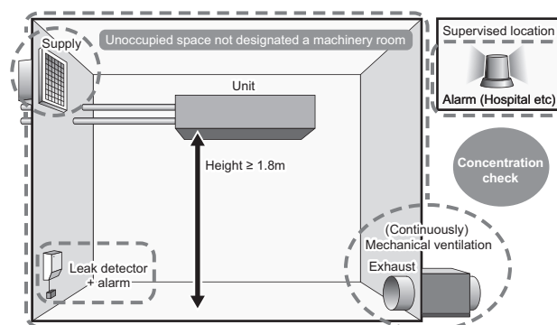
(1-5) Small room installation (Alarm + Ventilation)
