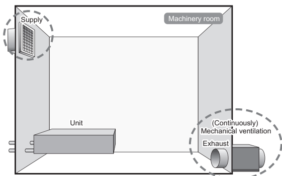
(1-1) Machinery room installation (Continuous ventilation)
