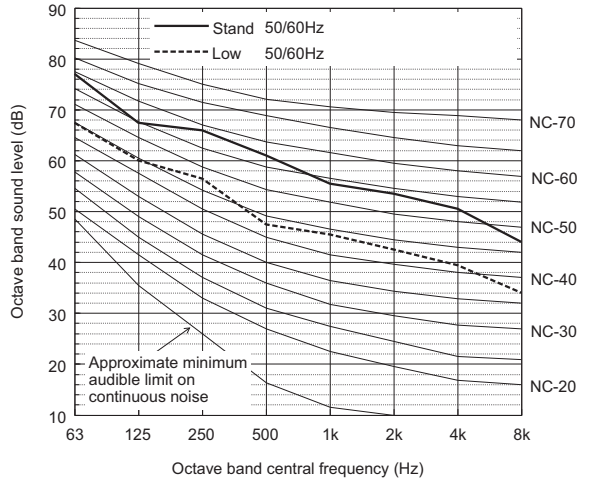
Sound level of PURY-EM500YNW-A1(-BS)
