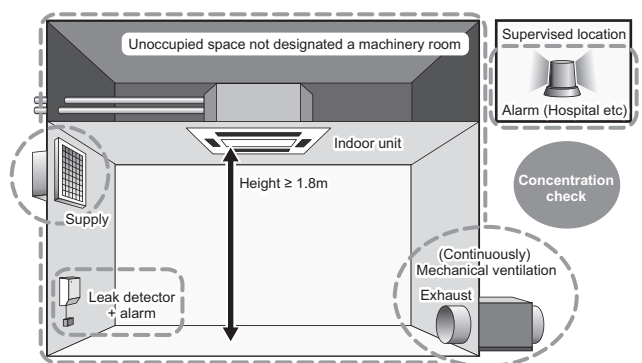
(2-4) Small room installation (Alarm + Ventilation)
