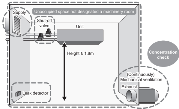
(1-6) Small room installation (Shut-off valves + Ventilation)
