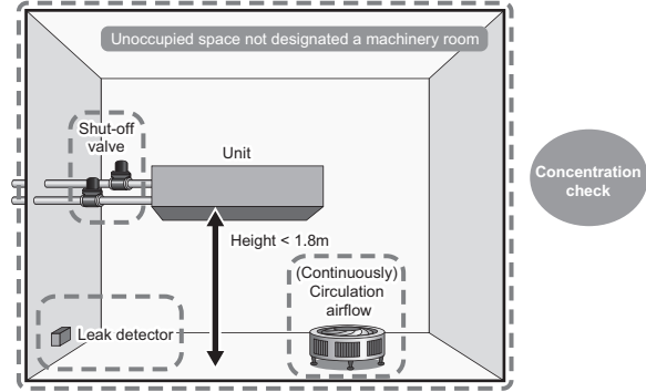
(1-14) Small room installation (Circulation + Shut-off valves)
