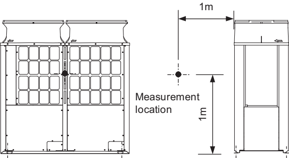
Measurement condition PURY-EM500YNW-A1(-BS)
