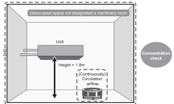
(1-9) Small room installation (Only circulation)
