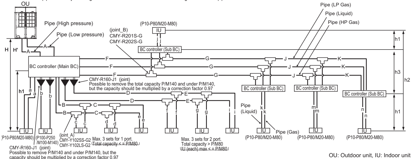
Fig. 12-2-5A Piping scheme
