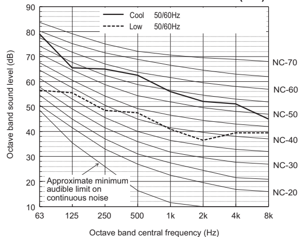
Sound level of PURY-P550YSNW-A2/TR2/RU2(-BS)
