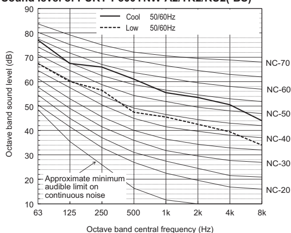
Sound level of PURY-P500YNW-A2/TR2/RU2(-BS)
