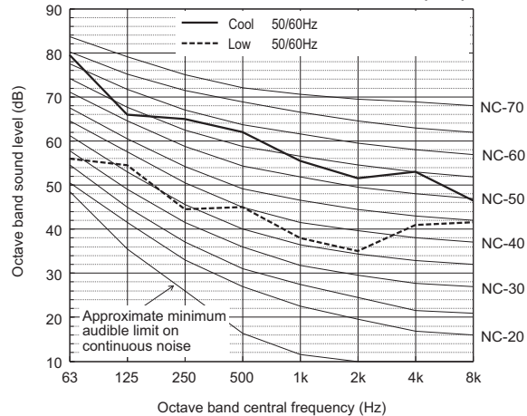
Sound level of PURY-P500YSNW-A2/TR2/RU2(-BS)
