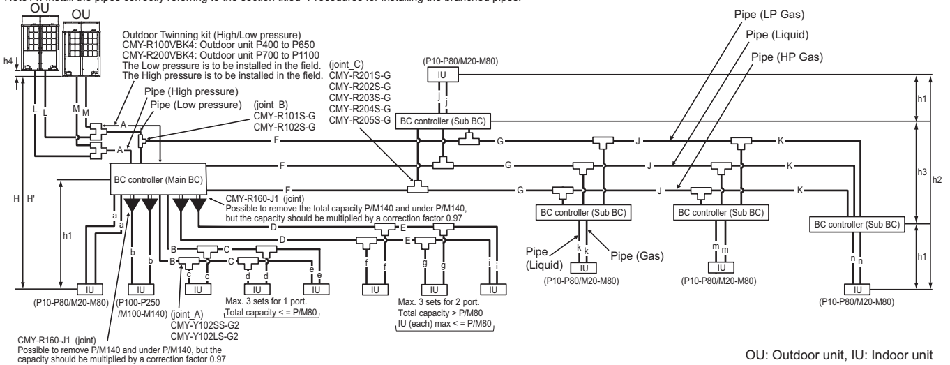
Fig. 12-2-3A Piping scheme
