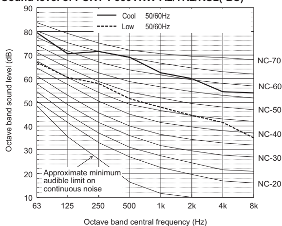
Sound level of PURY-P550YNW-A2/TR2/RU2(-BS)
