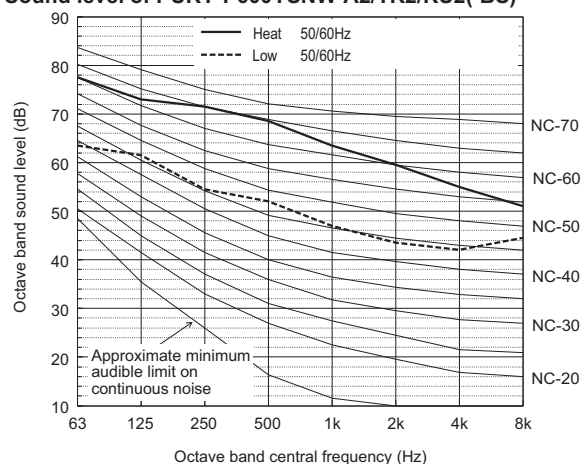
Sound level of PURY-P600YSNW-A2/TR2/RU2(-BS)
