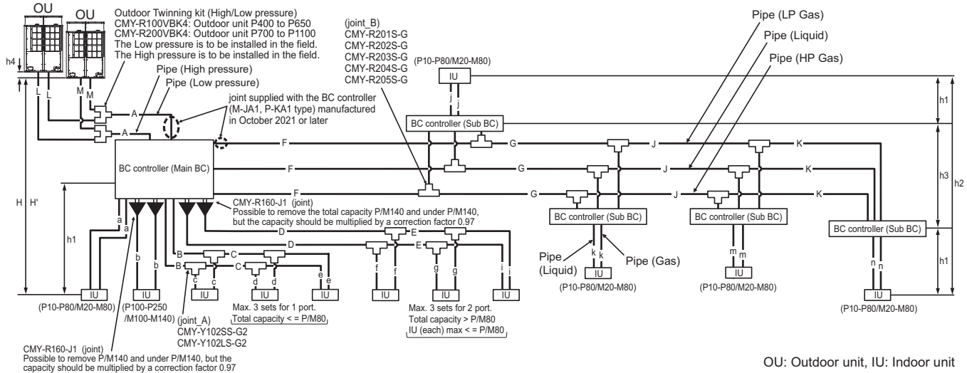
Fig. 12-2-6A Piping scheme
