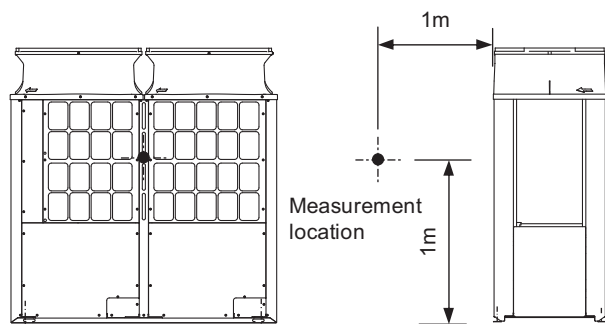
Measurement condition PURY-P500, 550YNW-A2/TR2/RU2(-BS)
