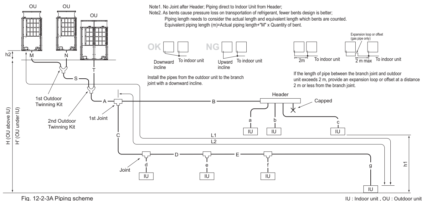
Fig. 12-2-3A Piping scheme
