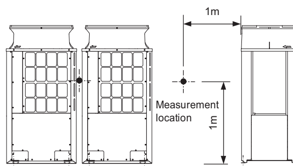
Measurement condition PUHY-P400, 450, 500, 550, 600YSNW-A2(-BS)
