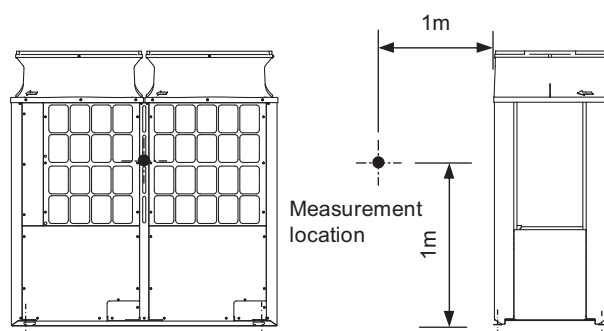
Measurement condition PUHY-P500YNW-A2(-BS)
