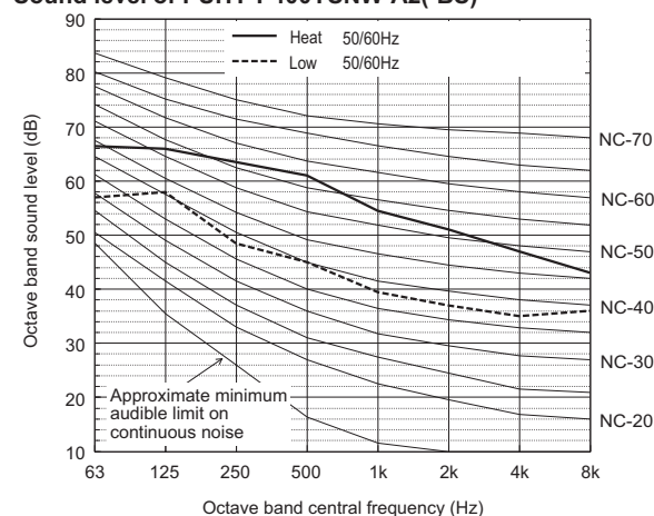
Sound level of PUHY-P400YSNW-A2(-BS)
