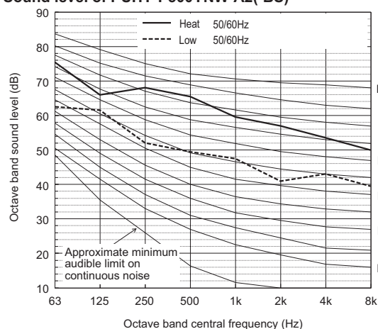
Sound level of PUHY-P500YNW-A2(-BS)
