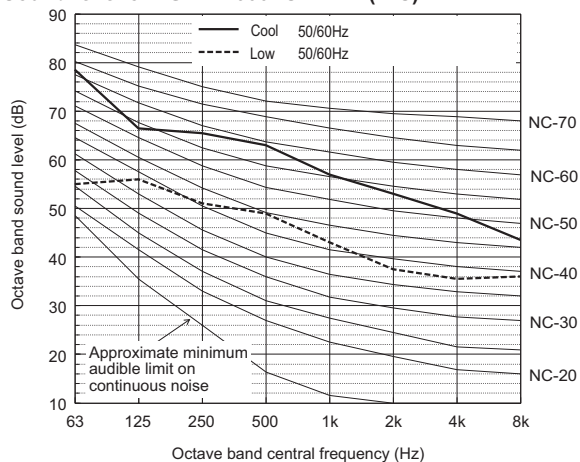
Sound level of PUHY-P600YSNW-A2(-BS)
