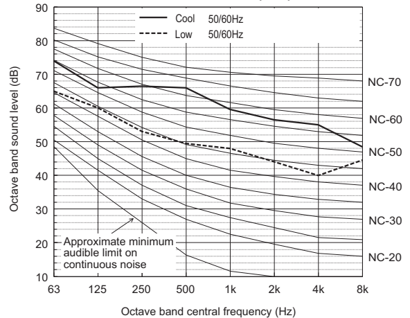
Sound level of PUHY-P650YSNW-A2(-BS)
