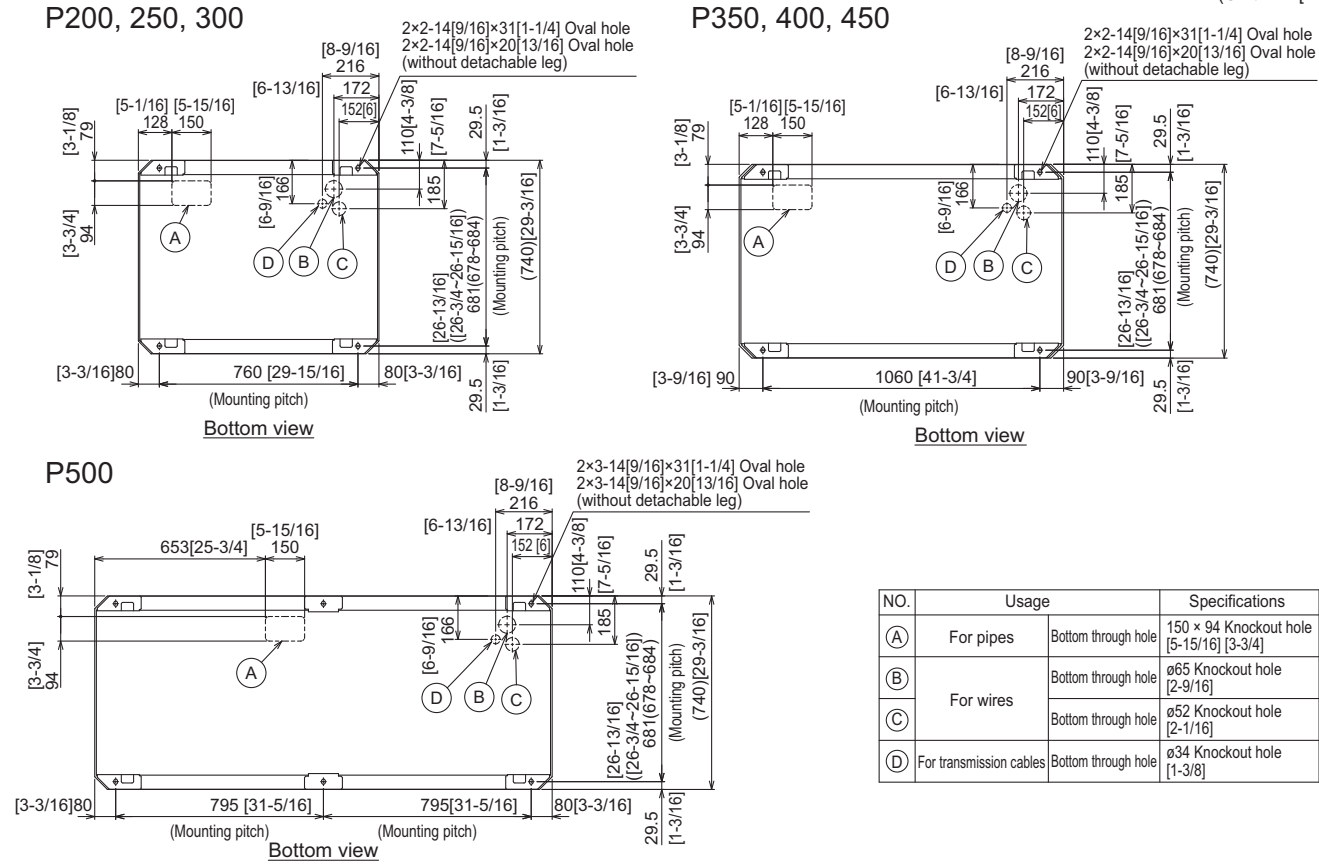
Installation base parallel to the unit's front panel
