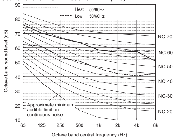
Sound level of PUHY-P550YSNW-A2(-BS)
