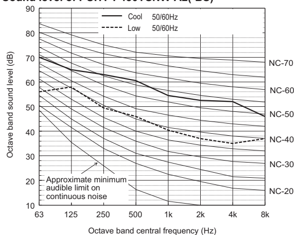
Sound level of PUHY-P450YSNW-A2(-BS)
