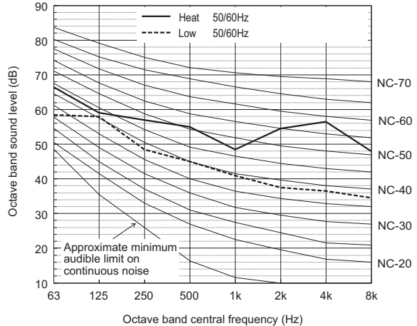
Sound level of PUHY-P250YNW-A2(-BS)
