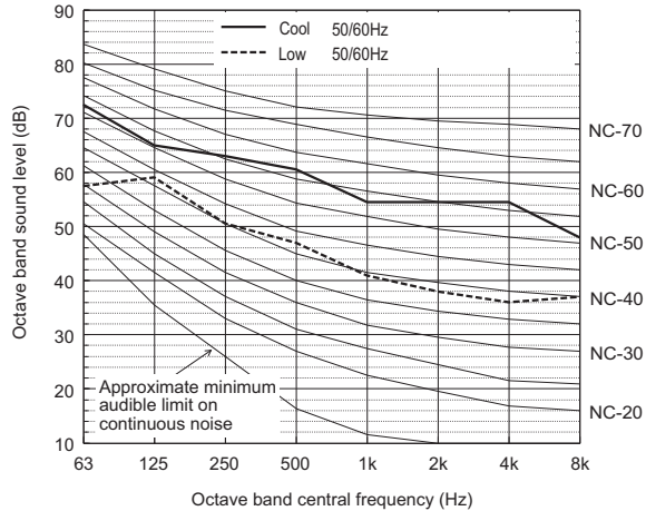
Sound level of PUHY-P500YSNW-A2(-BS)
