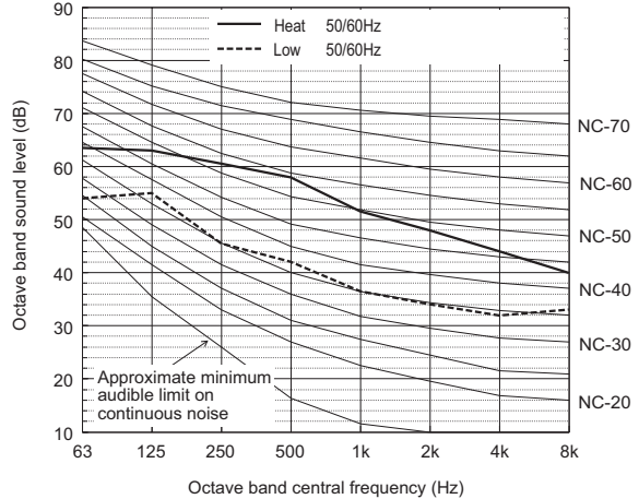
Sound level of PUHY-P200YNW-A2(-BS)
