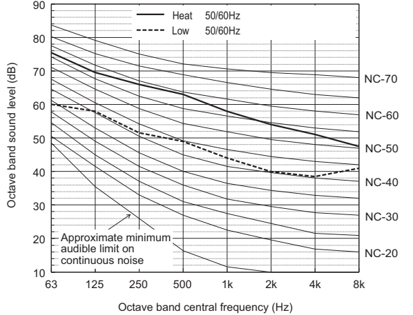
Sound level of PUHY-P300YNW-A2(-BS)
