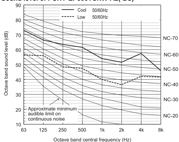
Sound level of PUHY-EP500YSNW-A2(-BS)
