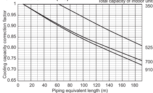
PUHY-EP700YSNW-A2(-BS)
