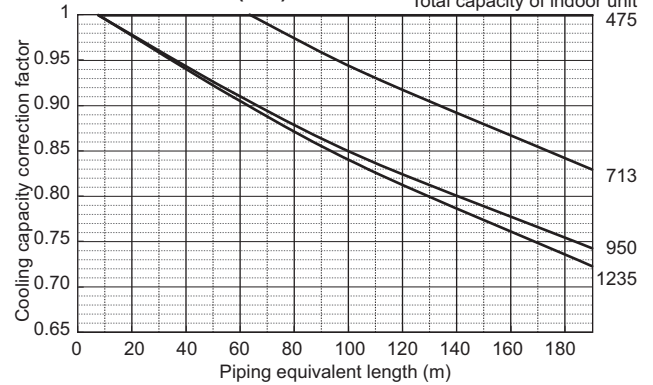
PUHY-EP950YSNW-A2(-BS)
