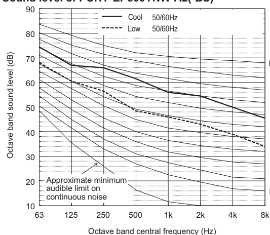
Sound level of PUHY-EP500YNW-A2(-BS)
