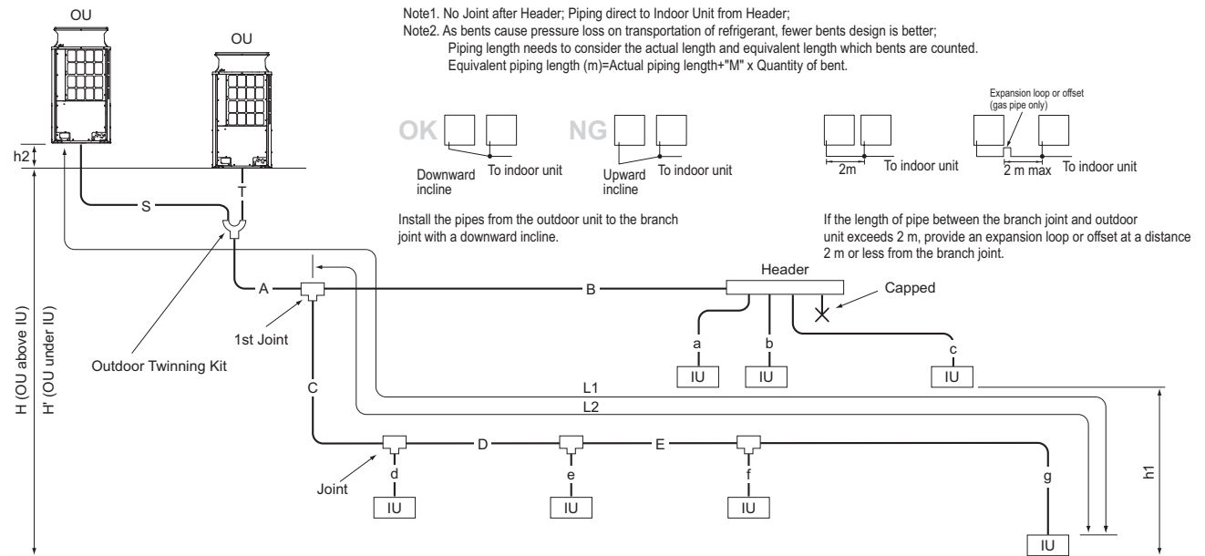
Fig. 12-2-2A Piping scheme
