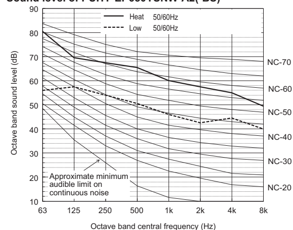
Sound level of PUHY-EP650YSNW-A2(-BS)
