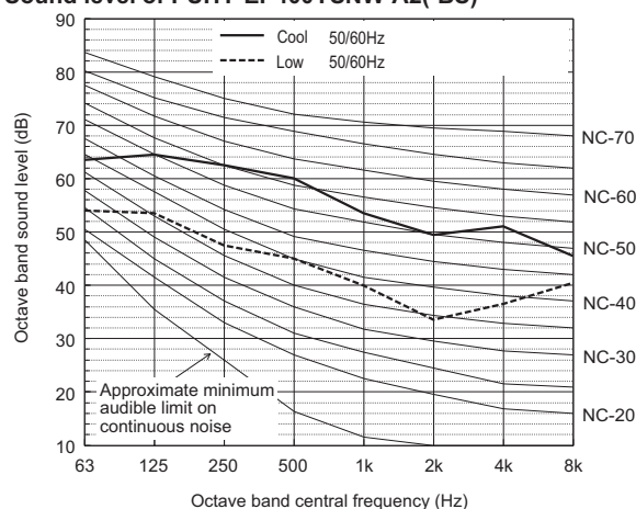
Sound level of PUHY-EP400YSNW-A2(-BS)
