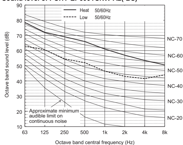
Sound level of PUHY-EP600YSNW-A2(-BS)
