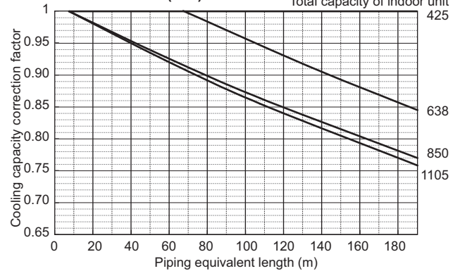
PUHY-EP850YSNW-A2(-BS)
