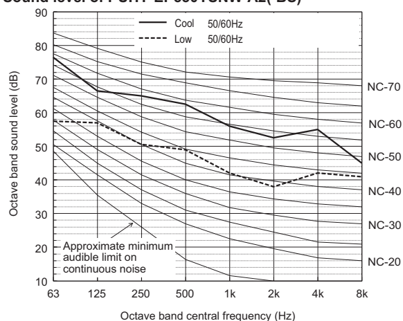
Sound level of PUHY-EP550YSNW-A2(-BS)
