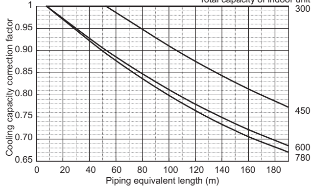
PUHY-EP600YSNW-A2(-BS)
