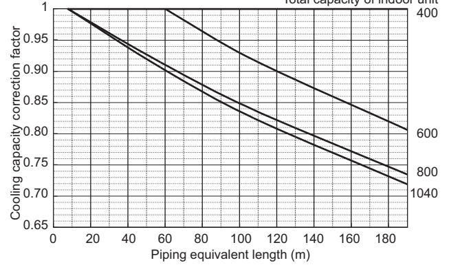
PUHY-EP800YSNW-A2(-BS)
