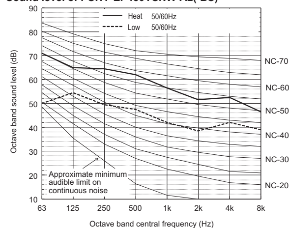
Sound level of PUHY-EP450YSNW-A2(-BS)
