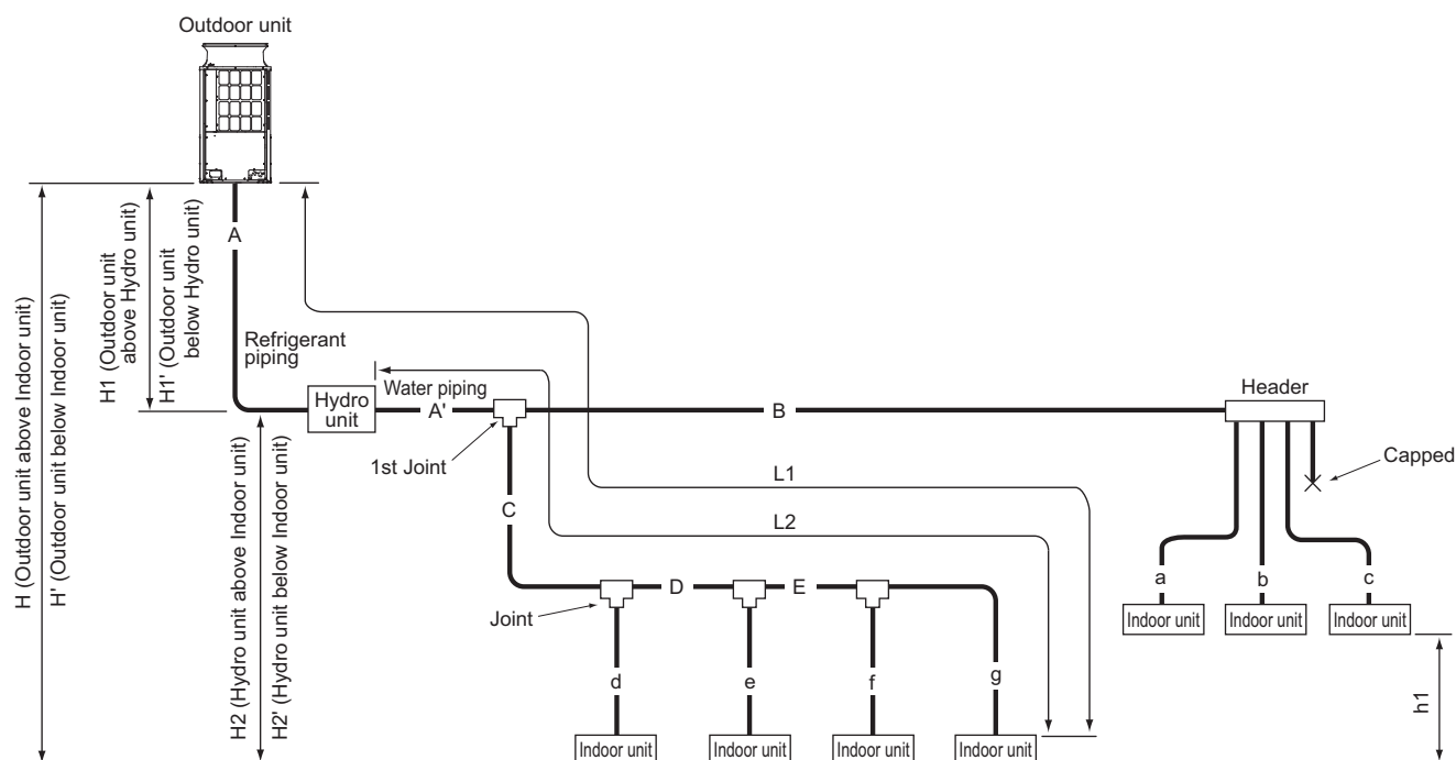
Fig. 11-2-1A Piping scheme
