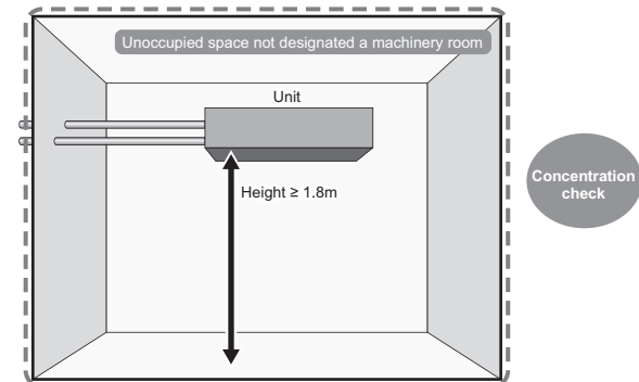
(1-2) Small room installation (No safety measures)
