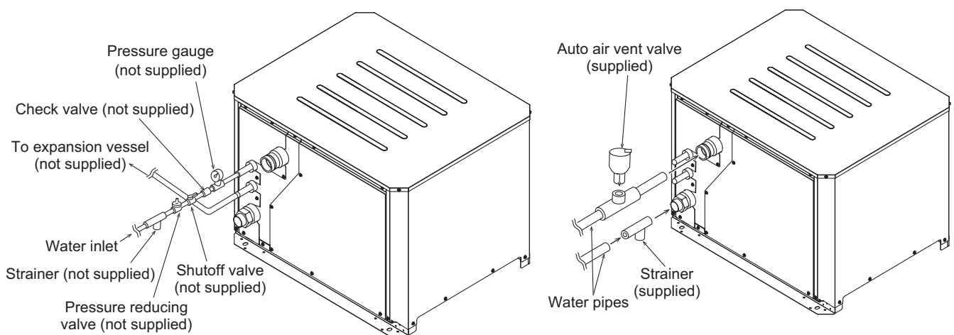
Hydro unit sample installation (*1)
