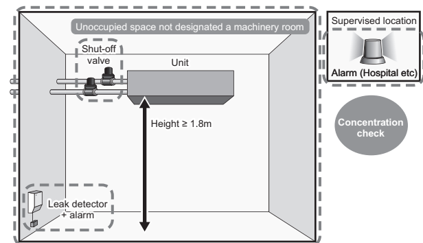
(1-4) Small room installation (Alarm + Shut-off valves)
