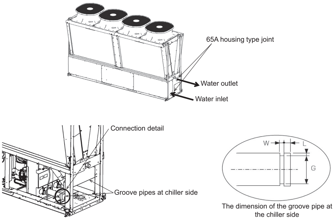
Victaulic standard groove specifications
