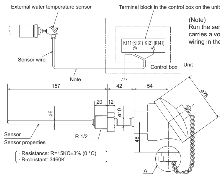
Terminal block for connection to the sensor
