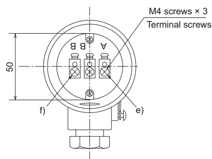
Terminal block for connection to the sensor
