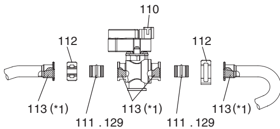
A Detail of 2-way valve
