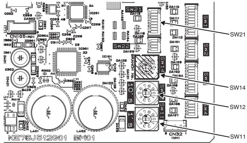
<Indoor controller board>
