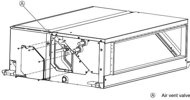
(A) Air vent valve
