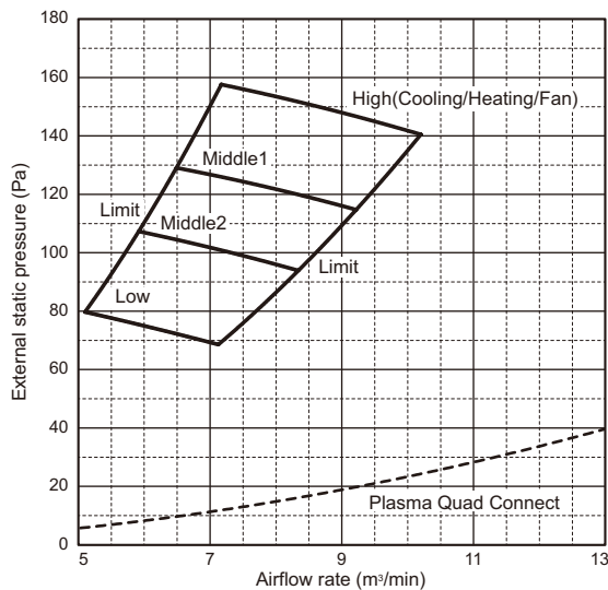
PEFY-M20, 25VMA(L)-A1 External static pressure : 150Pa Power source : 220-240V
