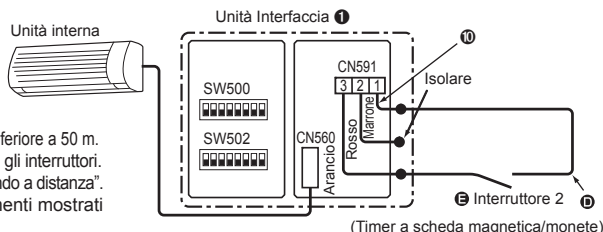
(Timer a scheda magnetica/monete)
